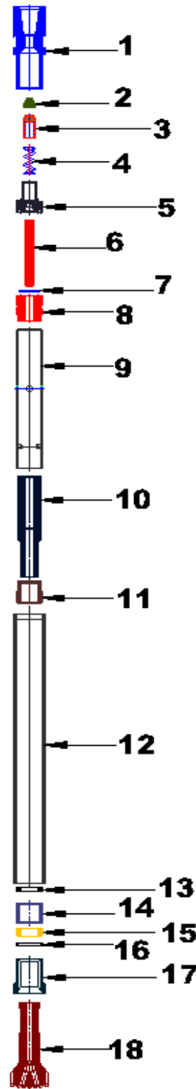
EXPLODE VIEW
